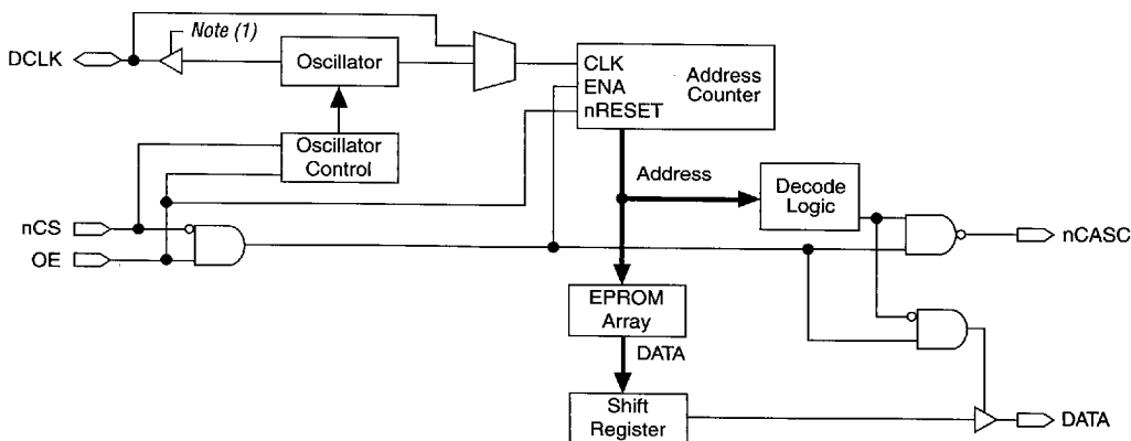
Figure 2. Configuration EPROM Block Diagram
