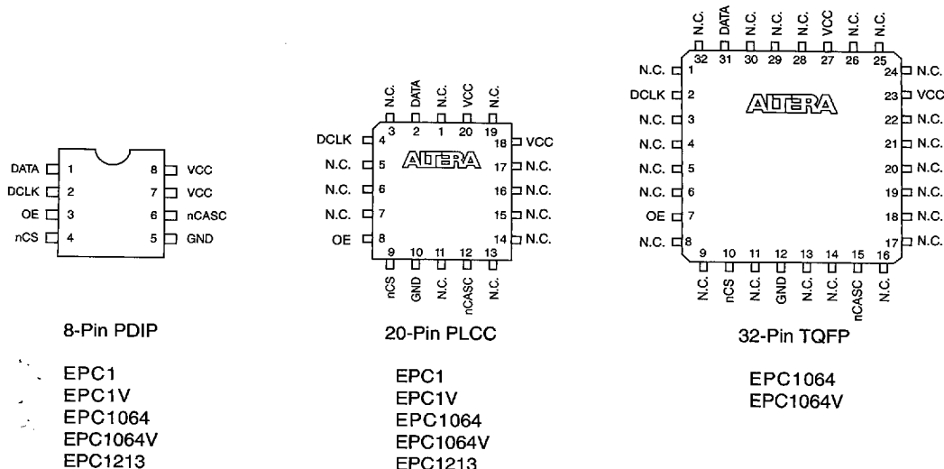
Figure 1. Configuration EPROM Package Pin-Out Diagrams
