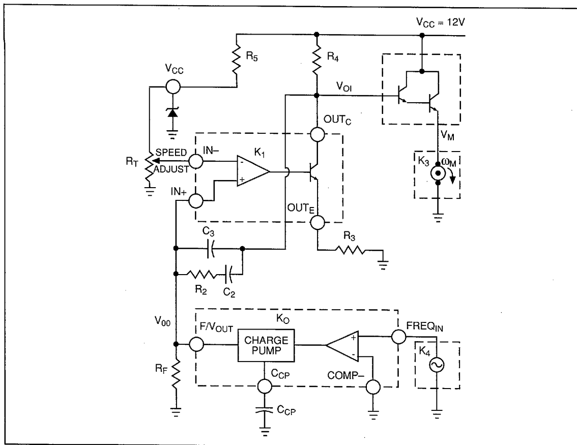
Figure 3: Motor Speed Control Block Diagram of CS-2917N8.
