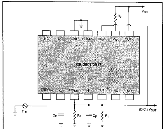
Figure 1: Application Diagram
