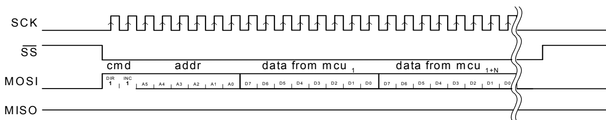
Figure 6. SPI Burst Write Sequence
