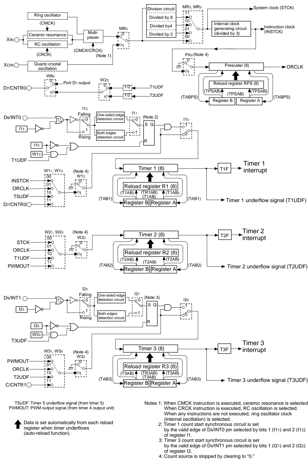
Fig. 25 Timer structure (1)
