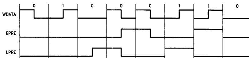
FIGURE 12. Example of EPRE and LPRE Outputs
