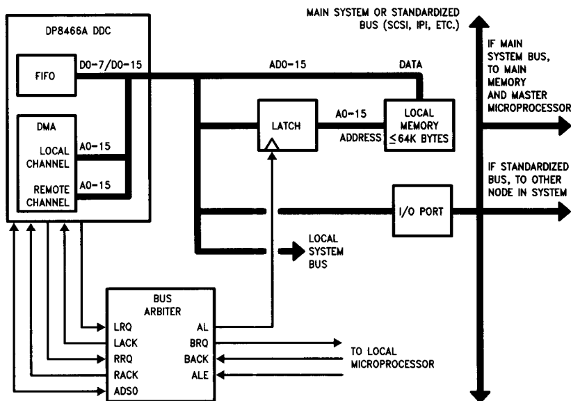
FIGURE 21. Dual System Bus, 16-Bit Address DMA
