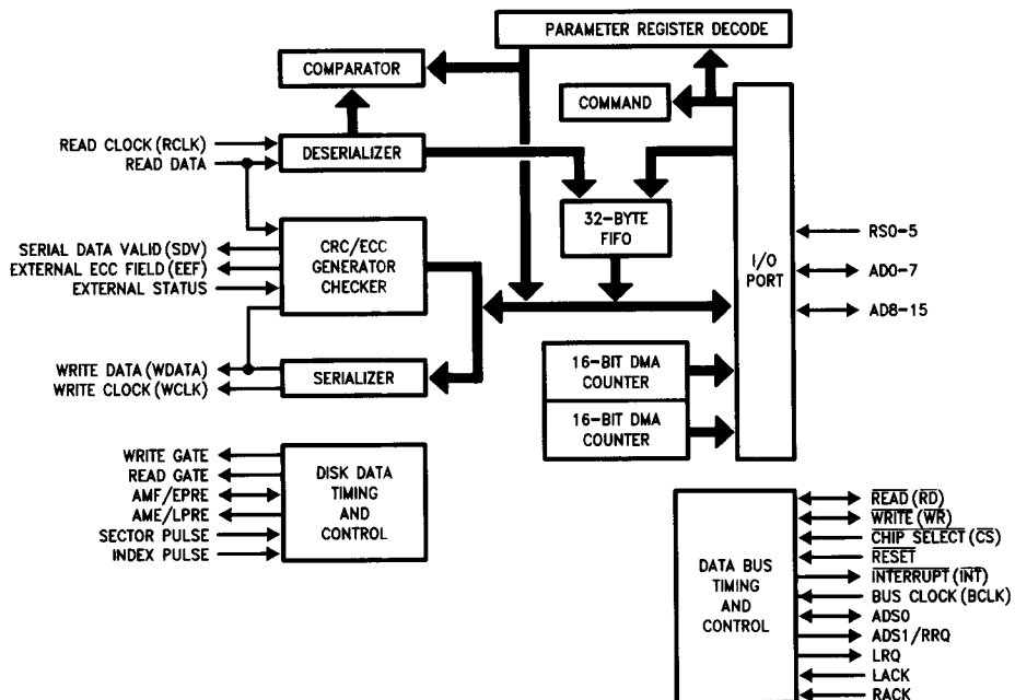
FIGURE 2. DDC
