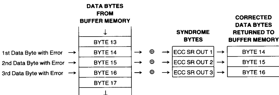
FIGURE 16. 48-Bit ECC Correction Process
