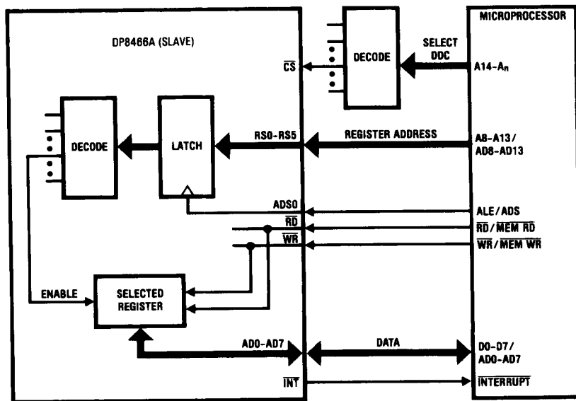
FIGURE 5. Microprocessor Access to DP8466A
