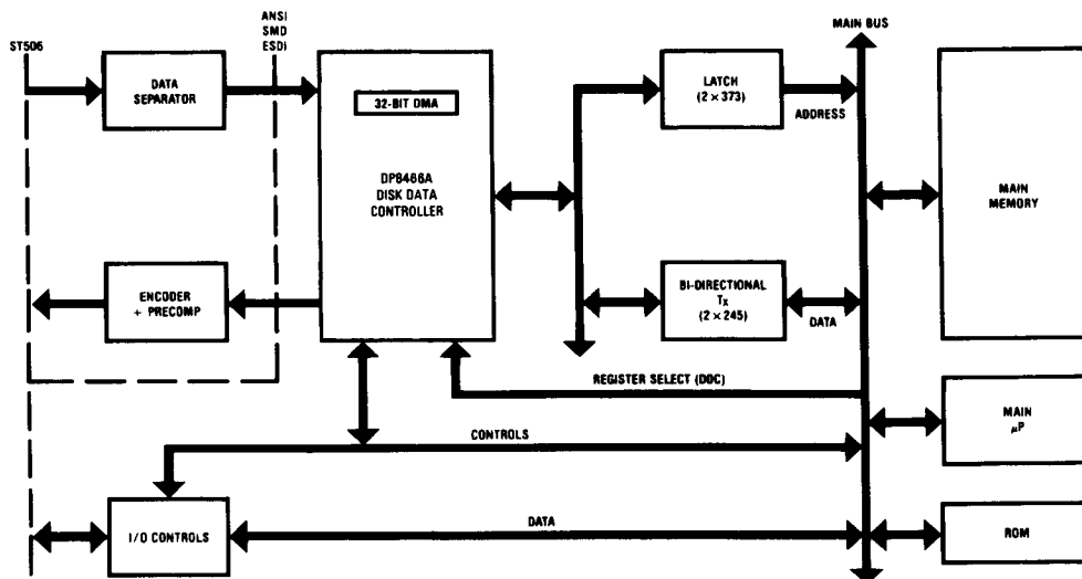
FIGURE 25. Low Cost System Configuration
