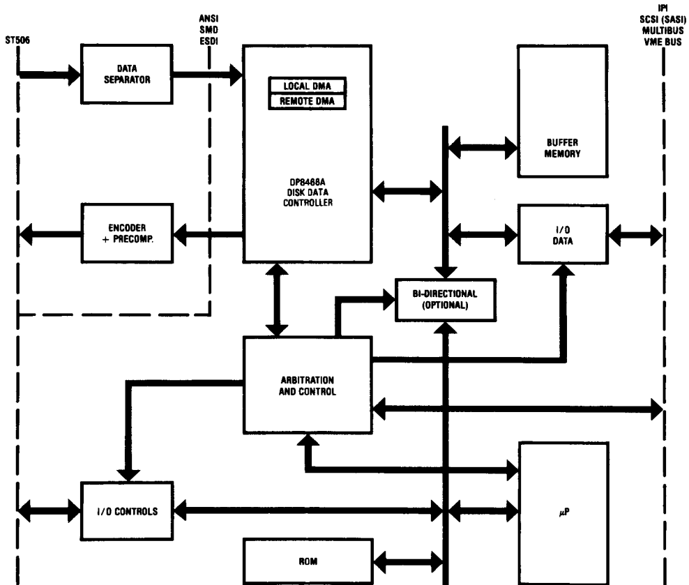
FIGURE 26. High Performance System
