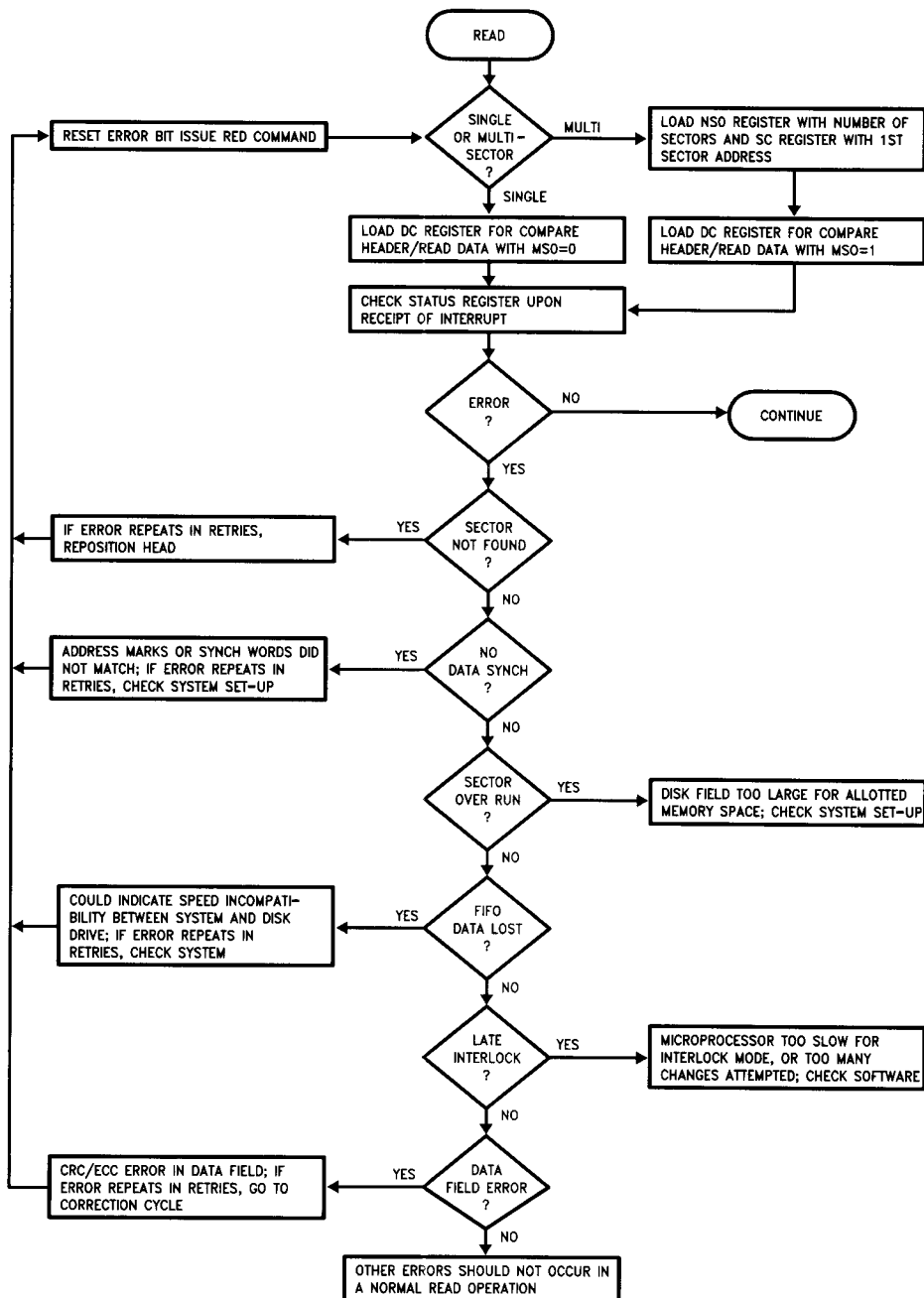
FIGURE 10. Simple Read Operation
