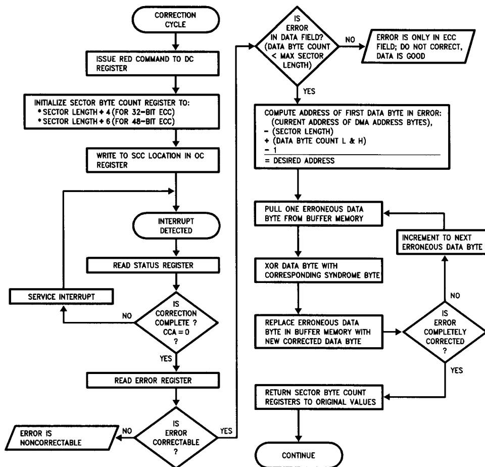
FIGURE 18. Correction Cycle Algorithm
