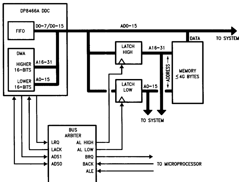
FIGURE 20. Single System Bus, 32-Bit Address DMA
