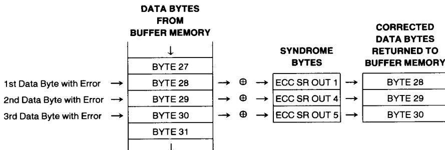
FIGURE 15. 32-Bit ECC Correction Process
