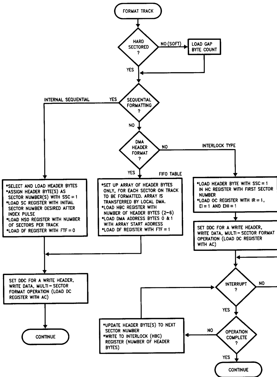
FIGURE 9. Format Track Algorithm
