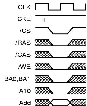
Fig.2 Mode register set command
