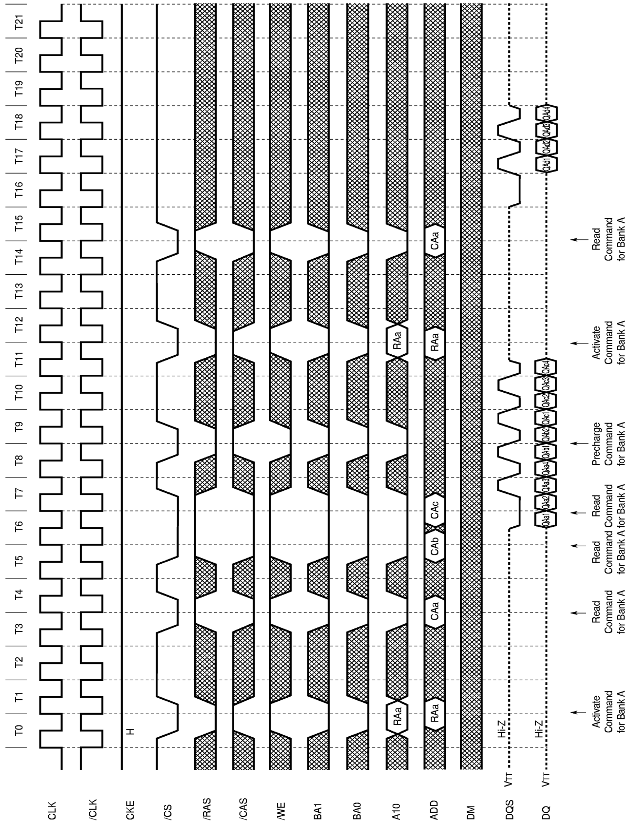
Random Column Read (Page with Same Bank) (2/2) (Burst Length = 4, /CAS Latency = 2.5)
