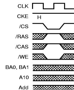
Fig.9 Burst stop command
