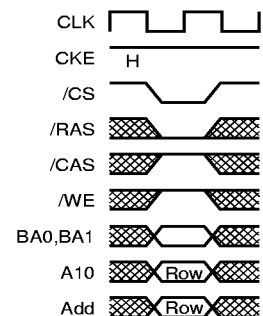
Fig.3 Bank activate command
