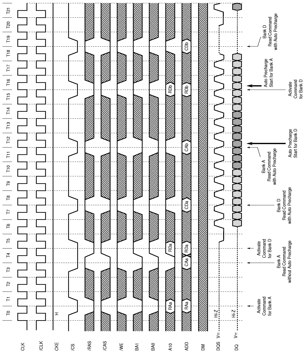
Auto Precharge after Read Burst (2/2) (Burst Length = 8, /CAS Latency = 2.5)
