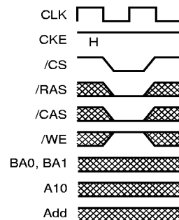
Fig.7 CBR (auto) refresh command
