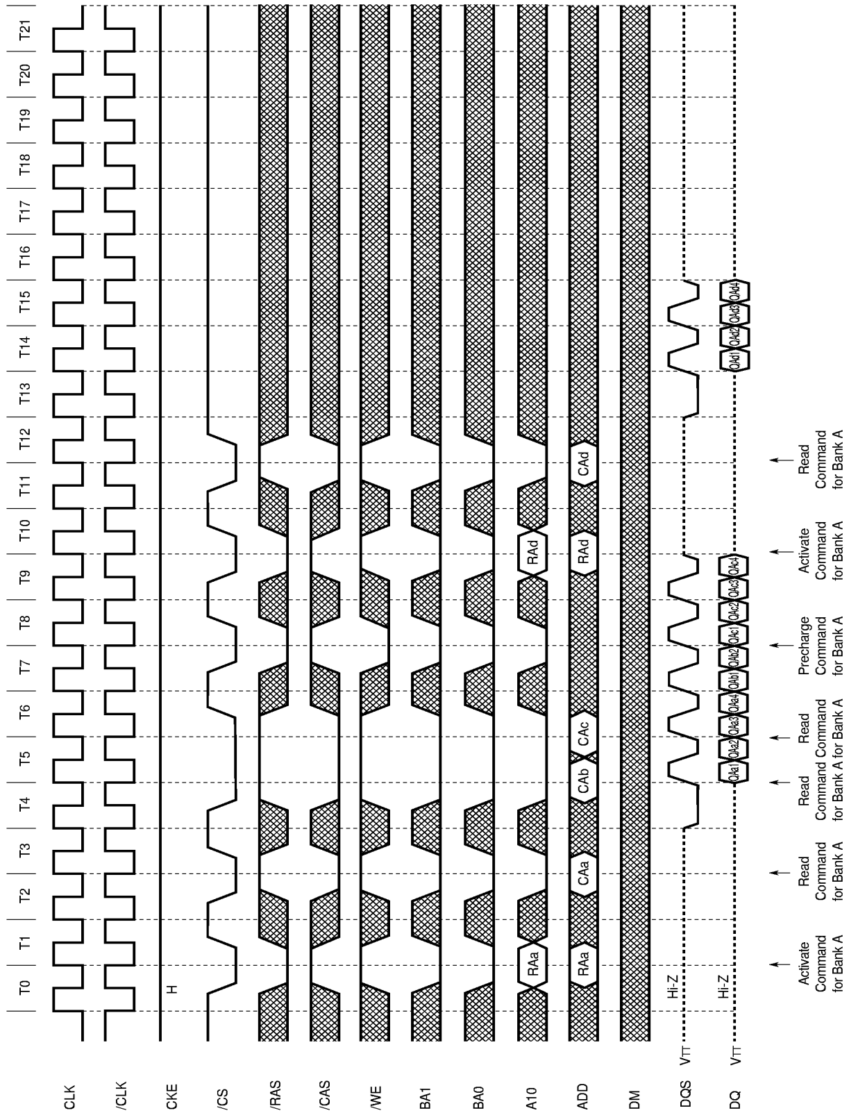
Random Column Read (Page with Same Bank) (1/2) (Burst Length = 4, /CAS Latency = 2)
