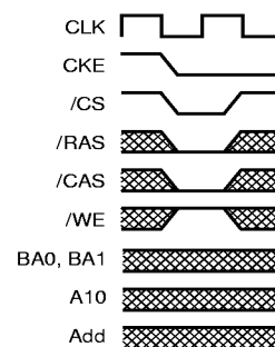
Fig.8 Self refresh entry command
