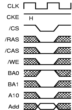
Fig.2 Mode register set command
