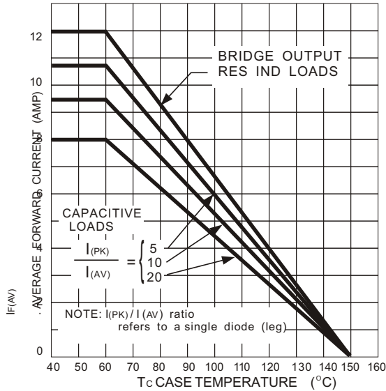
Figure 1 CURRENT DERATING
