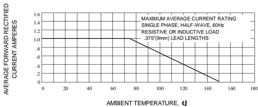
Fig. 5-FORWARD DERATING CURVE
