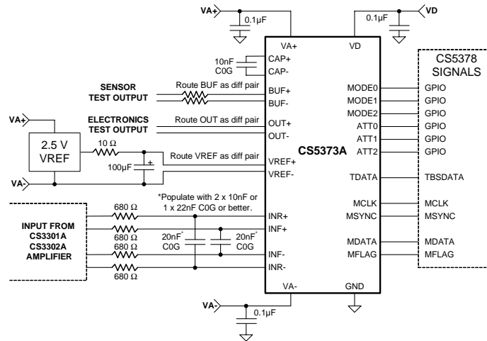
Figure 14. Analog Signals
