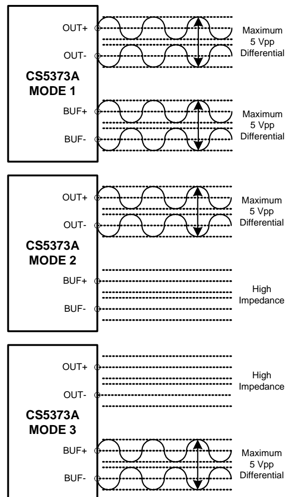
Figure 10. AC Differential Modes
