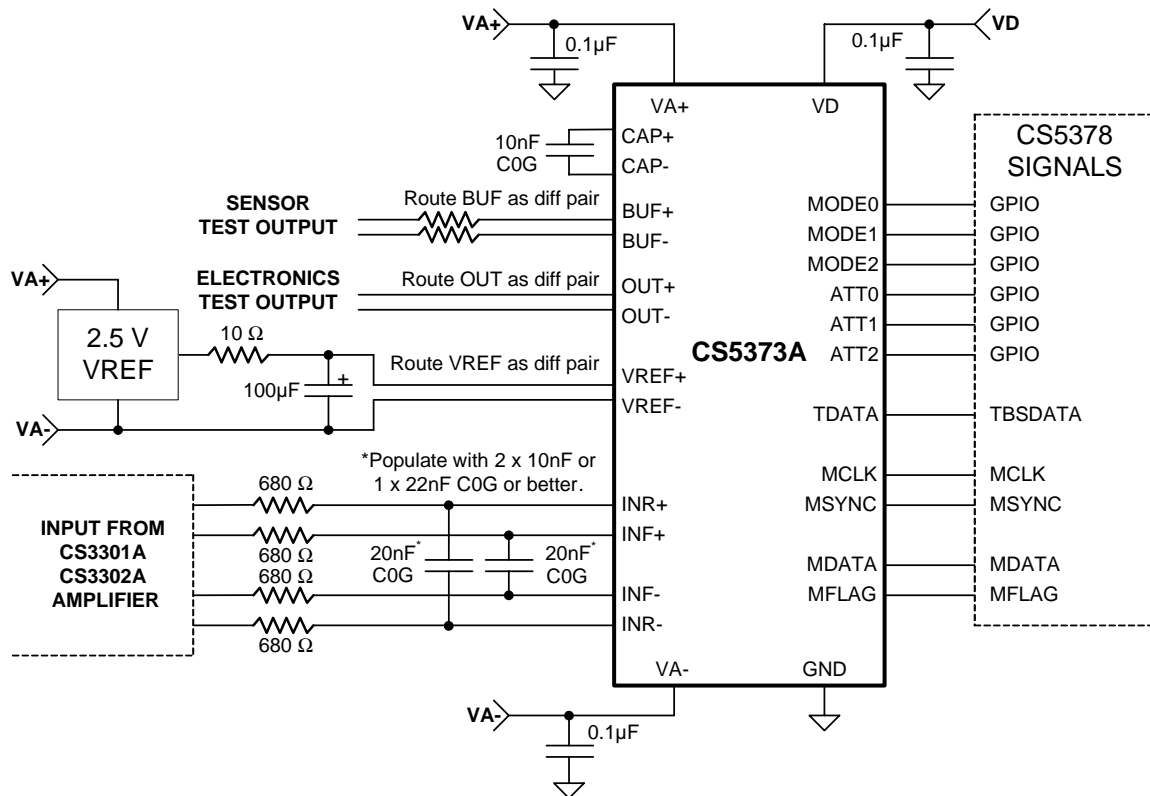
Figure 8. Connection Diagram
