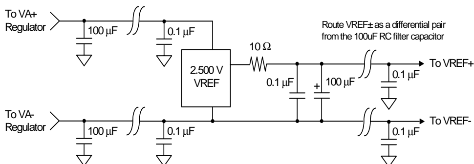
Figure 13. Voltage Reference Circuit
