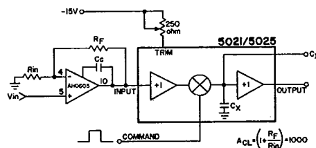
FIGURE 3: X1000 SAMPLE &amp; HOLD
