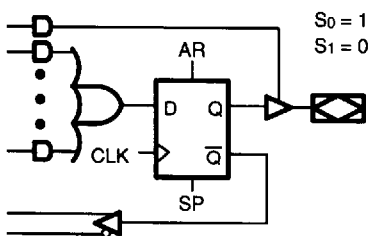
Registered/Active High
