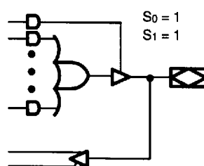
Combinatorial/Active High
