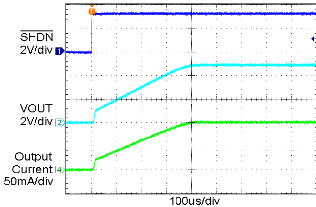
Figure 10. Power Up Waveform ( I_{OUT} = 100\text{ mA} )
