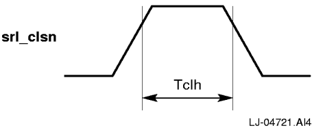
Figure 7 Serial Network Port Timing Diagram—Collision
