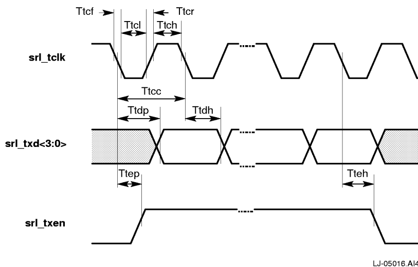
Figure 6 Serial Network Port Timing Diagram—Transmit
