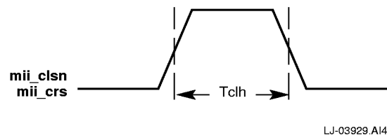
Figure 14 MII/SYM Port Timing Diagram—Carrier Sense and Collision
