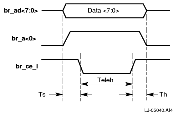
Figure 19 External Register Write Timing Diagram
