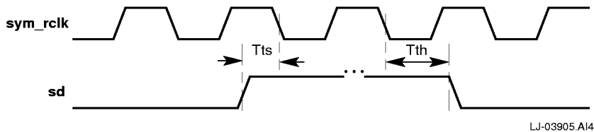
Figure 12 MII/SYM Port Timing Diagram—Signal Detect
