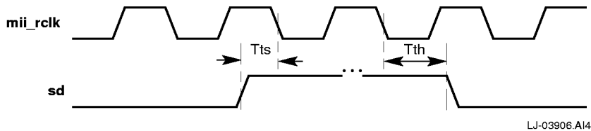
Figure 13 MII/SYM Port Timing Diagram—Receive Error
