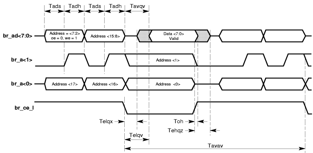
Figure 15 Boot ROM Read Timing Diagram
