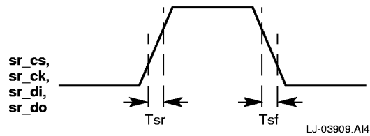
Figure 17 Serial ROM Port Timing Diagram
