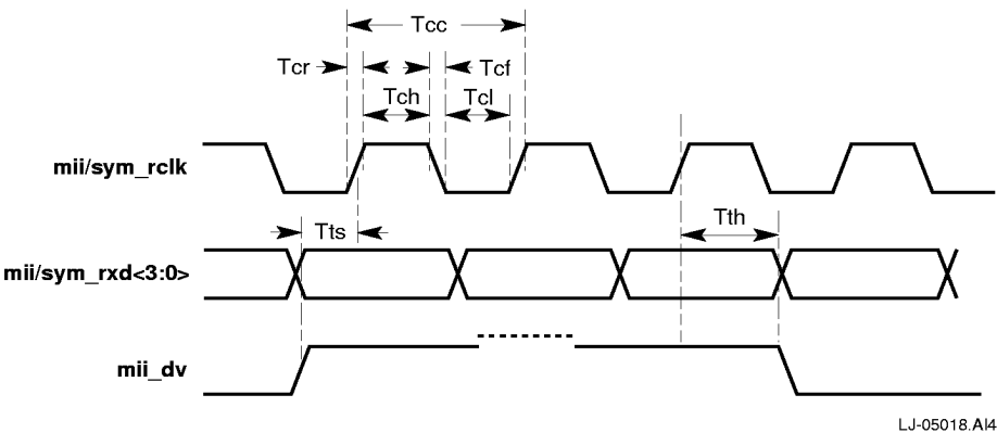
Figure 11 MII/SYM Port Timing Diagram—Receive
