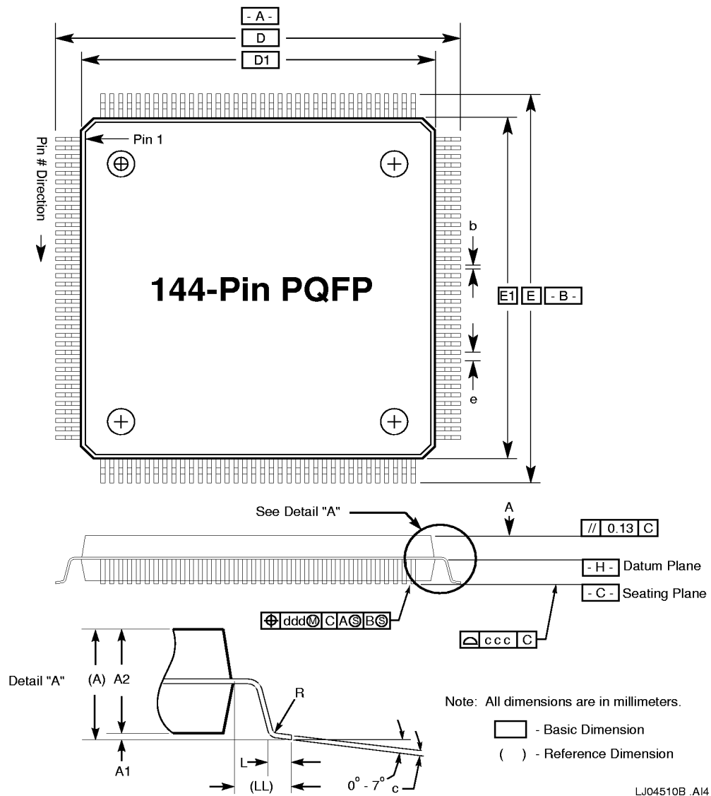
Figure 21 144-PIN PQFP Package
