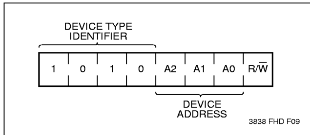
Figure 4. Slave Address
