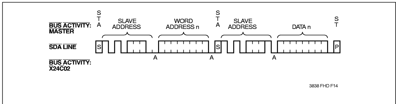
Figure 8. Random Read
