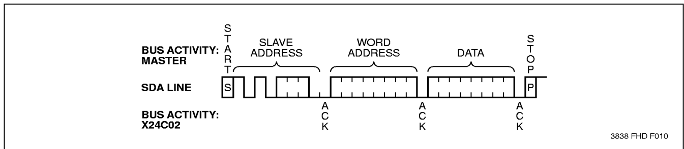
Figure 5. Byte Write
