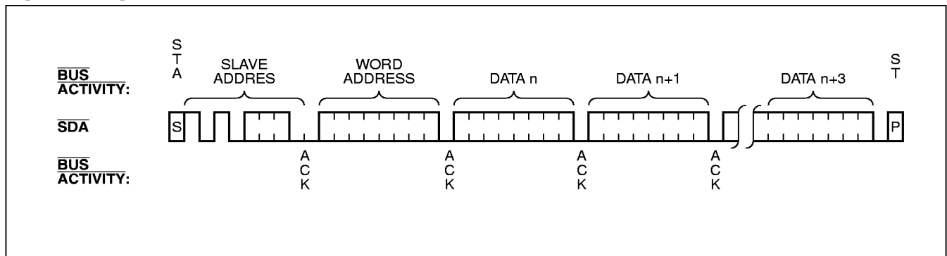
Figure 6. Page Write
