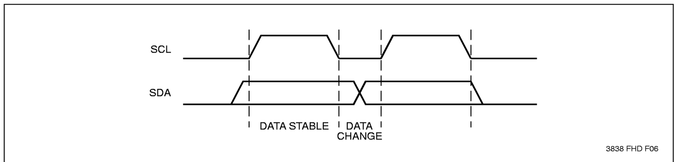
Figure 1. Data Validity
