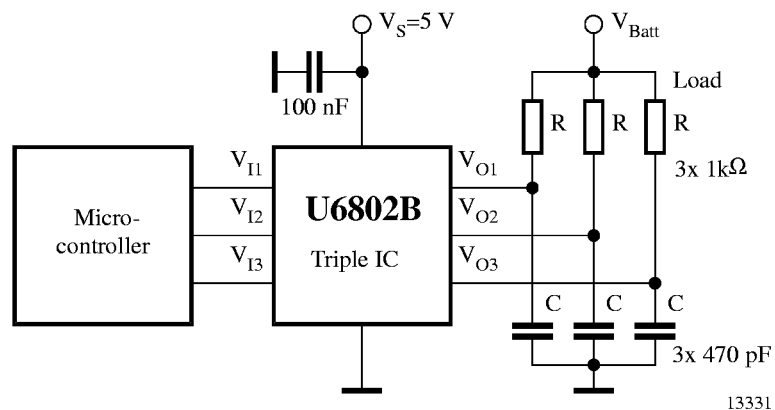
Figure 3. Application schematic
