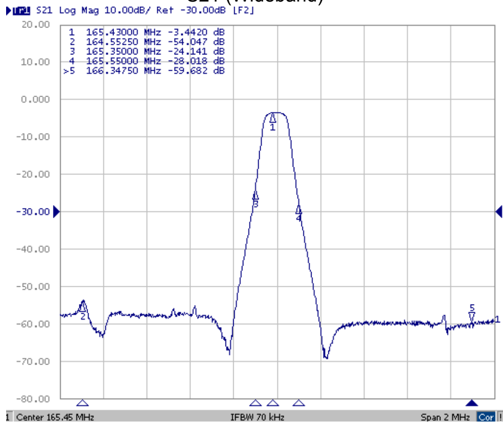
S21 (Wideband)
