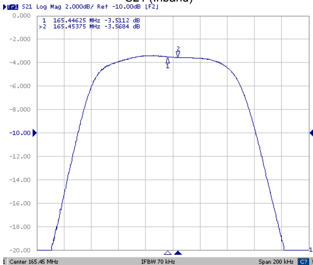
S21 (Inband)
