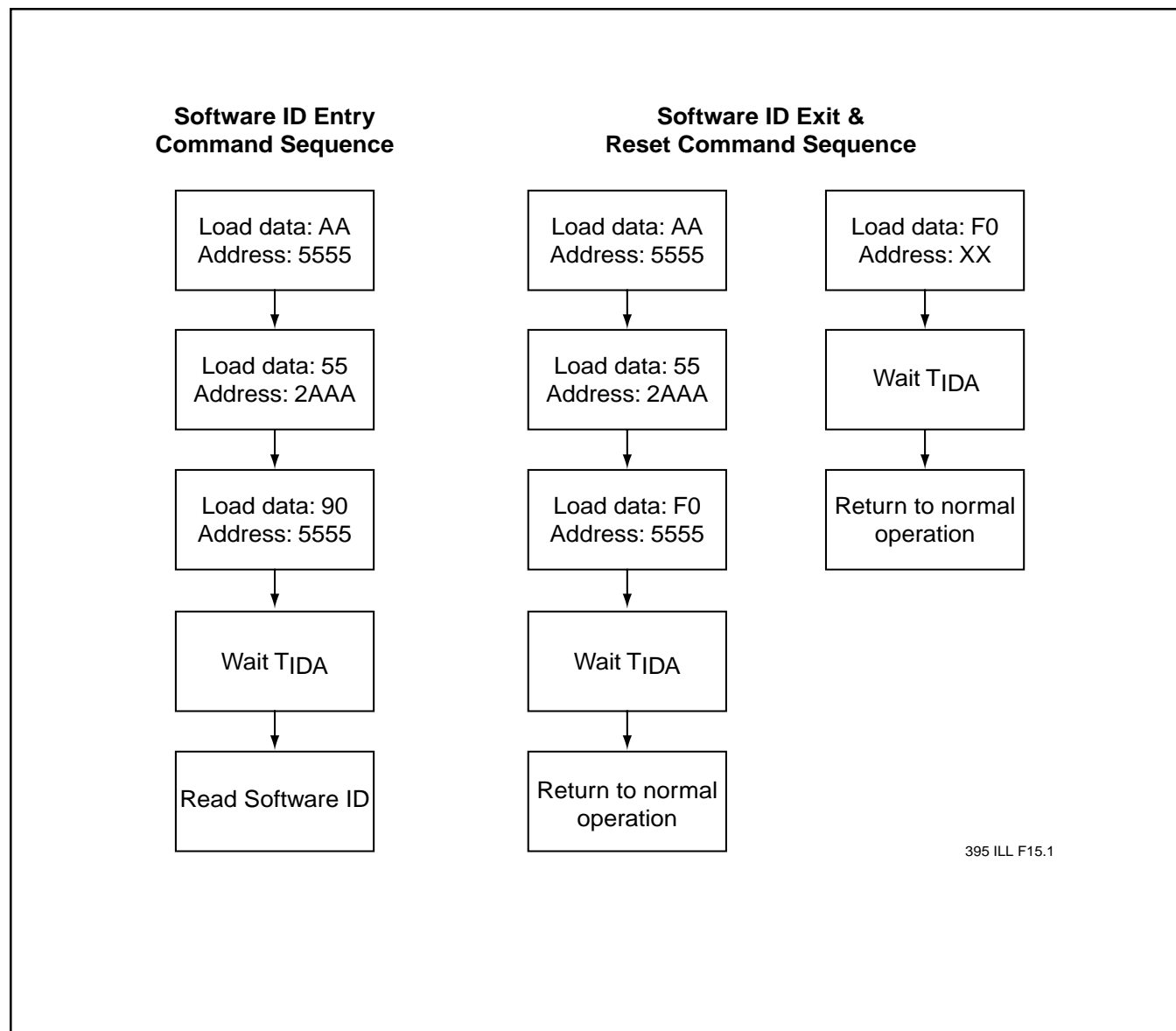
FIGURE 16: SOFTWARE ID COMMAND FLOWCHARTS
