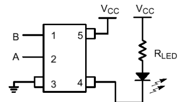
Figure 8. LED Driver
