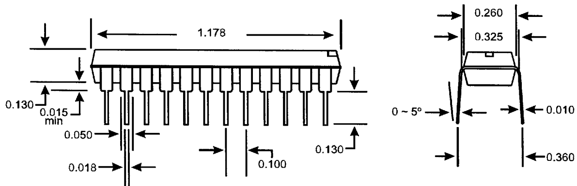
24-DIP Package
