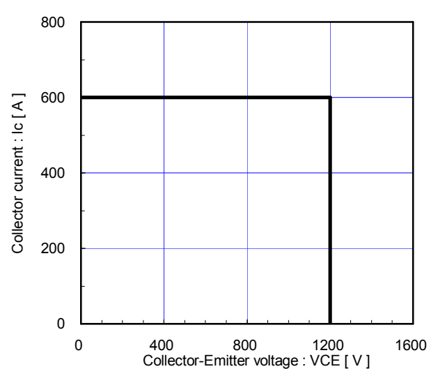
Reverse bias safe operating area (max.) +V_{GE}=15V, -V_{GE} \le 15V, R_G \ge 2.0\Omega, T_j \le 125^\circ C Stray inductance \le 100nH
