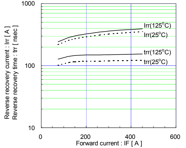
Reverse recovery characteristics (typ.) Vcc=600V, VGE=±15V, RG=2.0Ω
