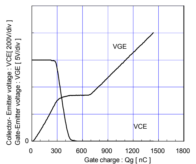
Dynamic Gate charge (typ.) Vcc=600V, Ic=300A, Tj=25°C
