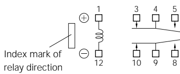
Non-latch type (not energized position)
