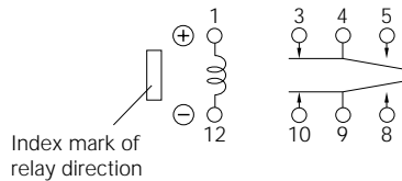
Non-latch type (not energized position)
