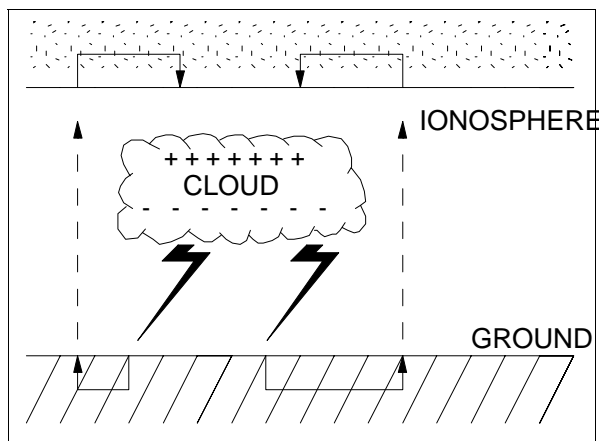
Figure 2 : Lightning phenomenon
