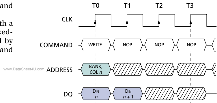
Figure 14 WRITE Burst
