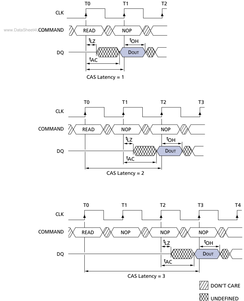
Figure 6 CAS Latency
