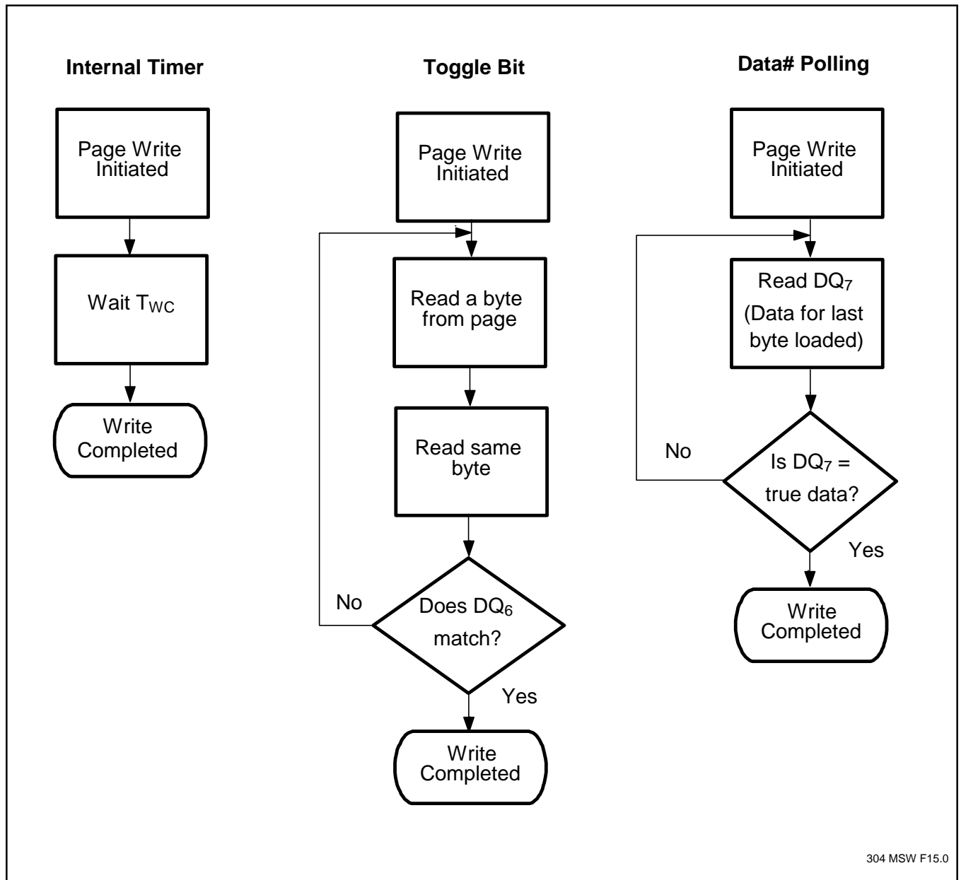
FIGURE 15: WAIT OPTIONS
