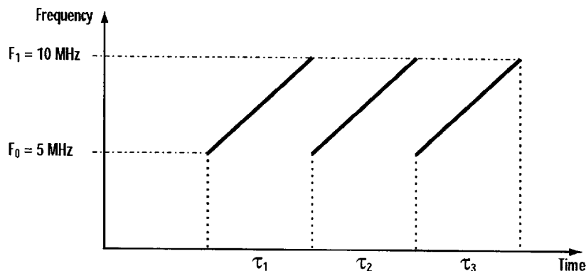
Figure 13. Q2368 Incrementing Chirp Example
