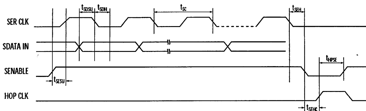
Figure 17. Q2368 Serial Mode Interface Timing Diagram
