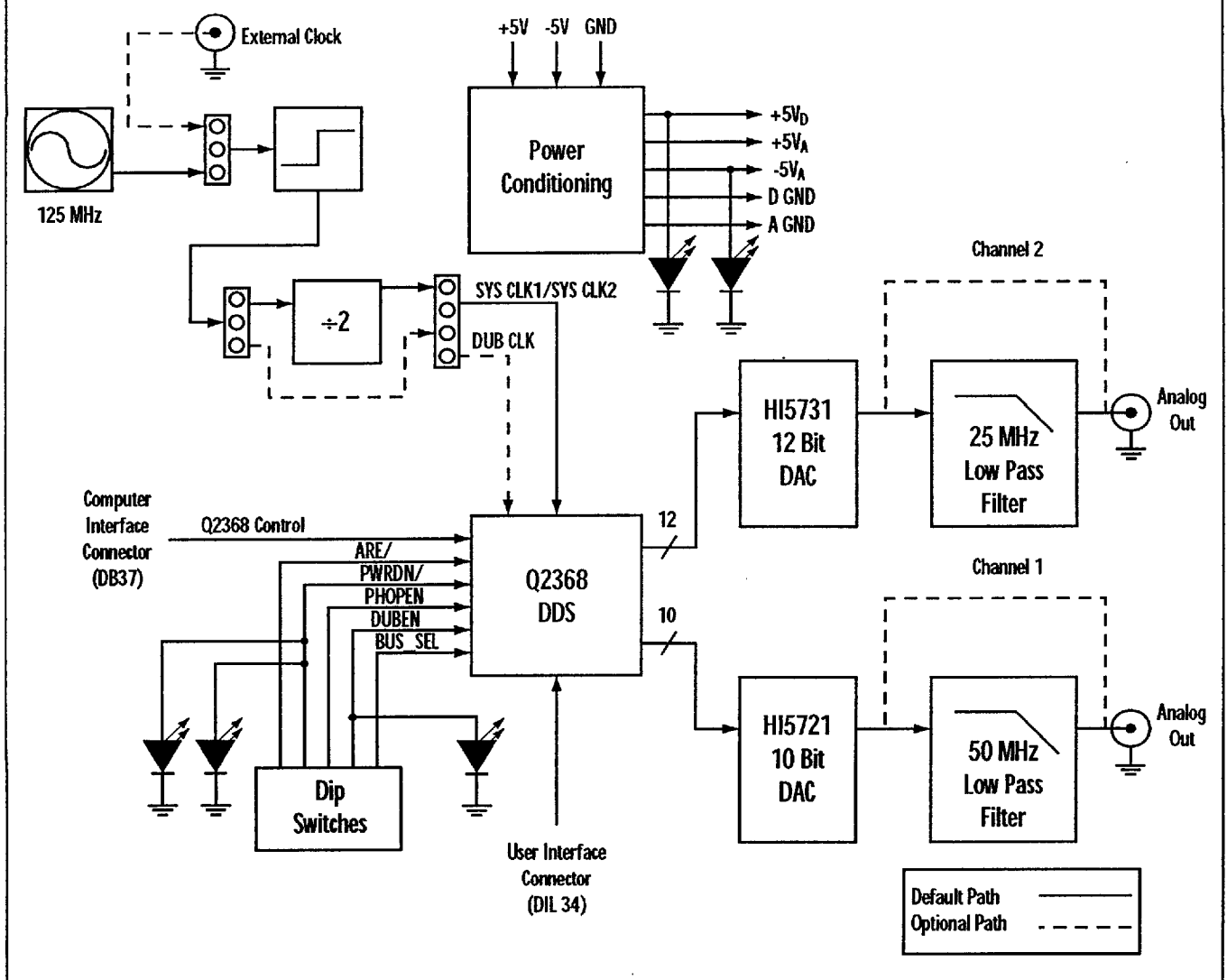
Figure 24. Q0315 Evaluation System Block Diagram
