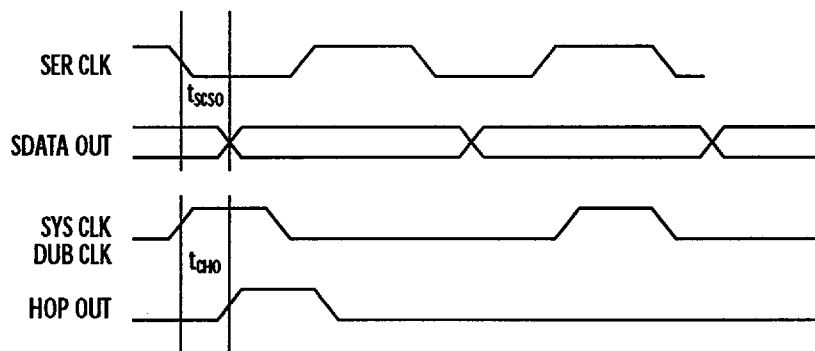
Figure 18. Q2368 Output Timing Diagram
