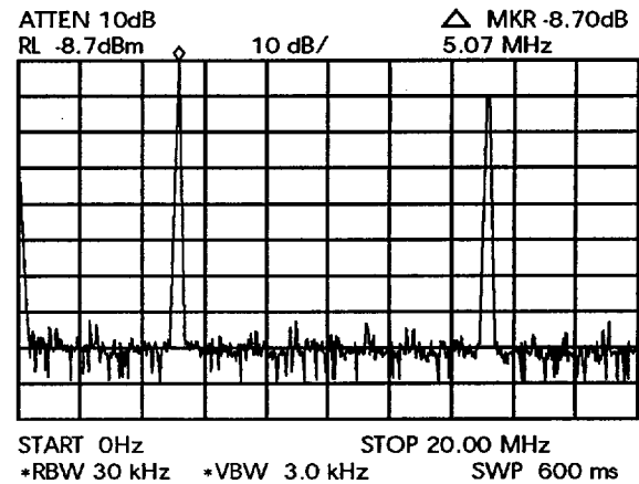
Figure 6. Q2368 Typical Spectrum with LPF Disabled (10-bit DAC)
