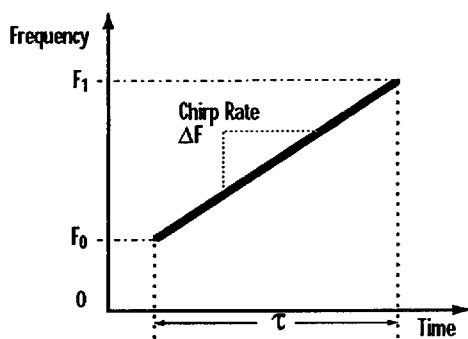
Figure 10. Q2368 Linear Chirp Waveform Example
