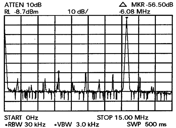
Figure 5. Q2368 Typical Spectrum with NRC Disabled (10-bit DAC)
