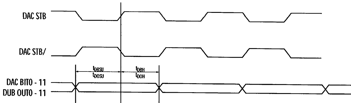
Figure 21. Q2368 DAC Interface Timing Diagram
