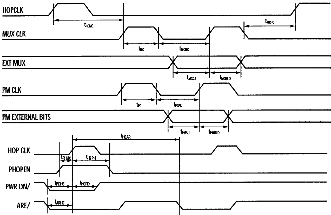
Figure 20. Q2368 External Control Timing Diagram
