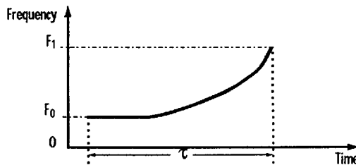
Figure 11. Q2368 Piecewise-Linear Chirp Waveform
