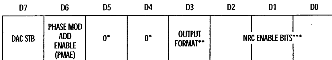
Figure 3. Q2368 Asynchronous Mode Control (AMC) Register
