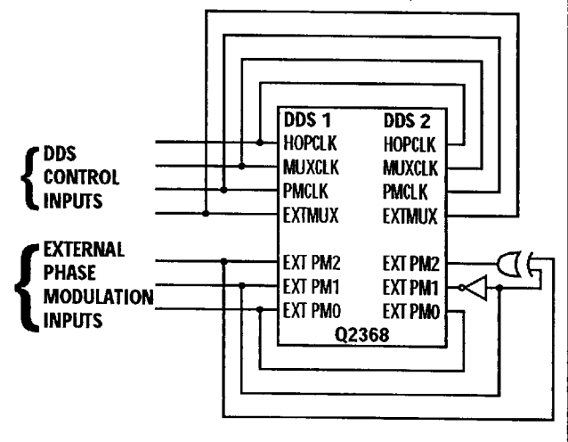
Figure 8b. Q2368 Quadrature Signal Implementation (Phase Modulated Quadrature Oscillator)
