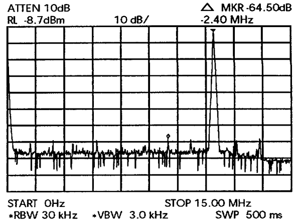
Figure 4. Q2368 Typical Spectrum with NRC Enabled (10-bit DAC)
