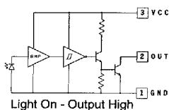
OPL550-OC (Open-Collector Output) Buffer
