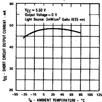
Short Circuit Output Current vs. Ambient Temperature
