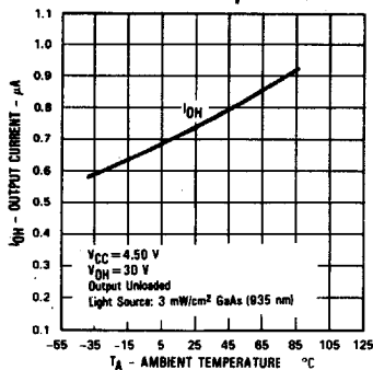
Output Current (High) vs Ambient Temperature
