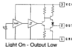
OPL551-OC (Open-Collector Output) Inverter
