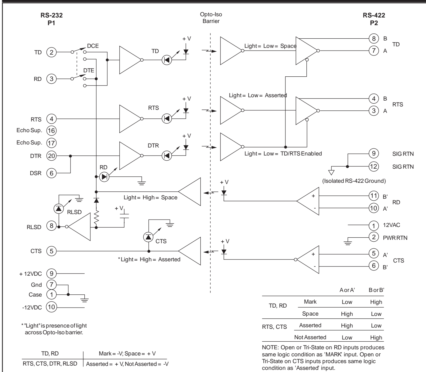
Figure 1. LDM422 Logic Diagram
