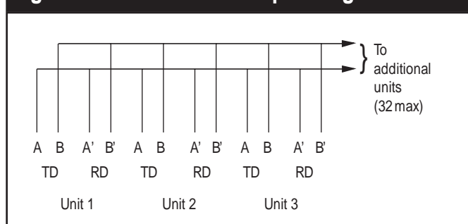
Figure 3. LDM422 Multidrop Wiring Connection
