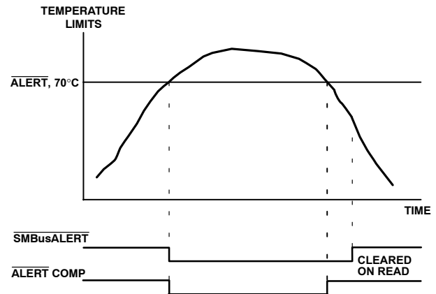
Figure 30. \overline{\text{ALERT}} Comparator and SMBus \overline{\text{ALERT}} Outputs
