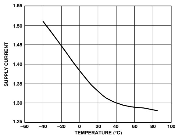
Figure 14. Supply Current vs. ADM1034 Temperature
