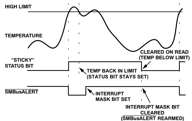
Figure 31. Handling SMBus \overline{\text{ALERT}}
