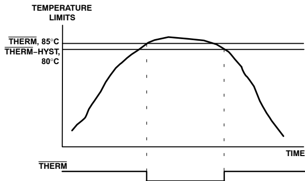
Figure 32. THERM Behavior
