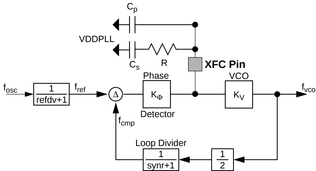
Figure B-3 Basic PLL functional diagram
