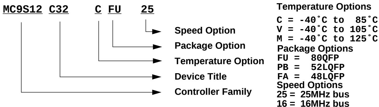
Figure 0-1 Order Part number Coding
