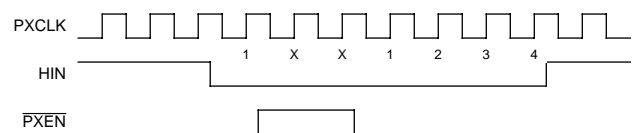
Figure 11. Effective PXCLK Cycles (4 Effective Cycles)
