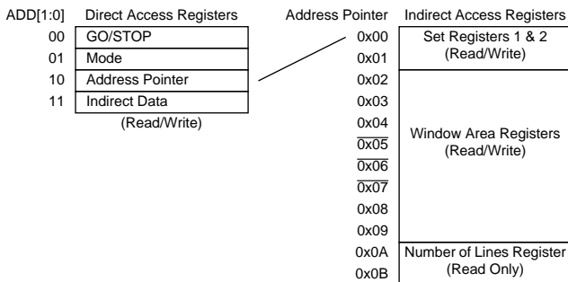
Figure 3. Control Registers
