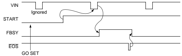
Figure 20. Processing Controlled by START Signal in Single Frame Compression Mode
