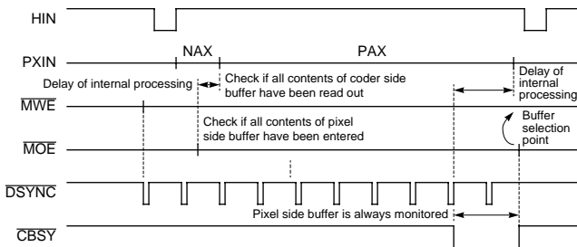
Figure 28. Expansion Operation When CBSY is Asserted but the Line is Not Ignored
