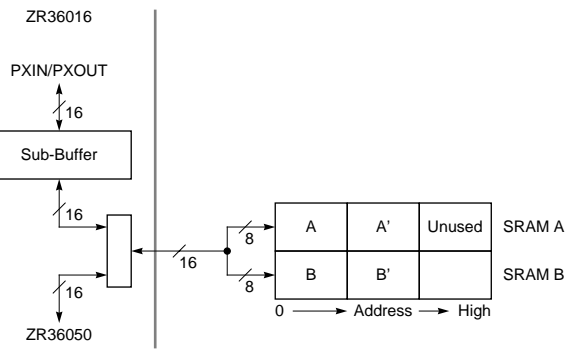
Figure 29. Strip Buffer Interface
