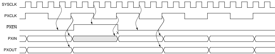
Figure 7. PXCLK = SYSCLK/4
