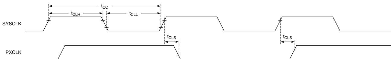
Figure 36. Clock Timing
