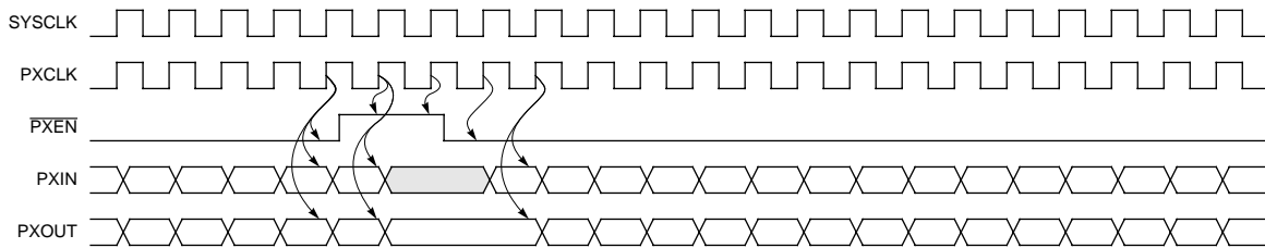
Figure 8. PXCLK = SYSCLK
