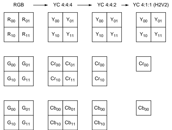
Figure 13. Decimation Flow
