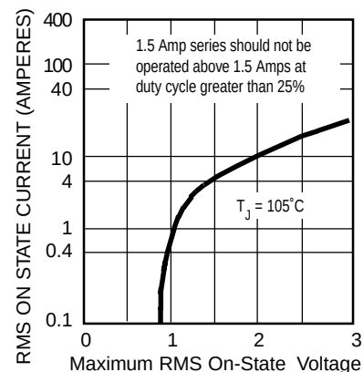
CLASS 230/231
