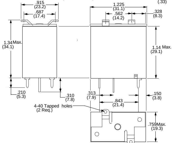
STYLE R1C4
