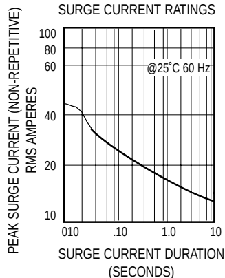
SURGE CURRENT RATINGS
