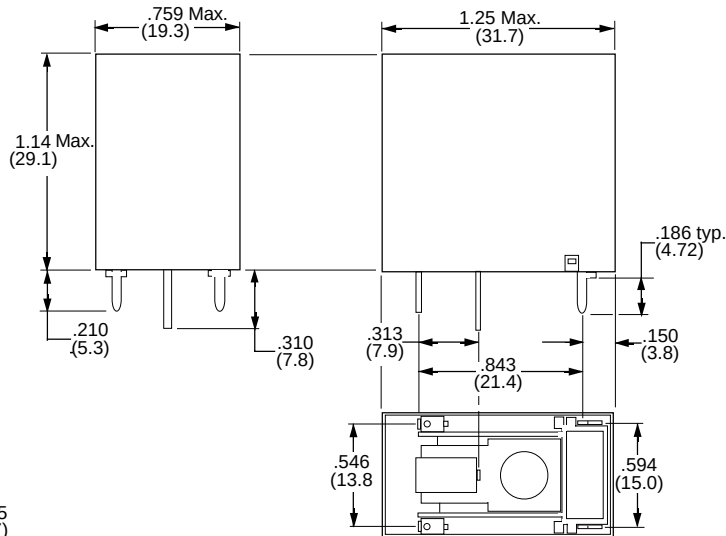
STYLE RE1C1
