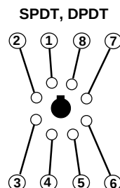
70-464-1 PANEL/DIN MOUNT SOCKET Struthers-Dunn Equivalent Part Number 75224
