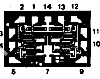
SCL4002B 56 x 37 mils
