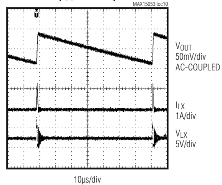
SWITCHING WAVEFORM IN SKIP MODE ( I_{OUT} = 10mA )
