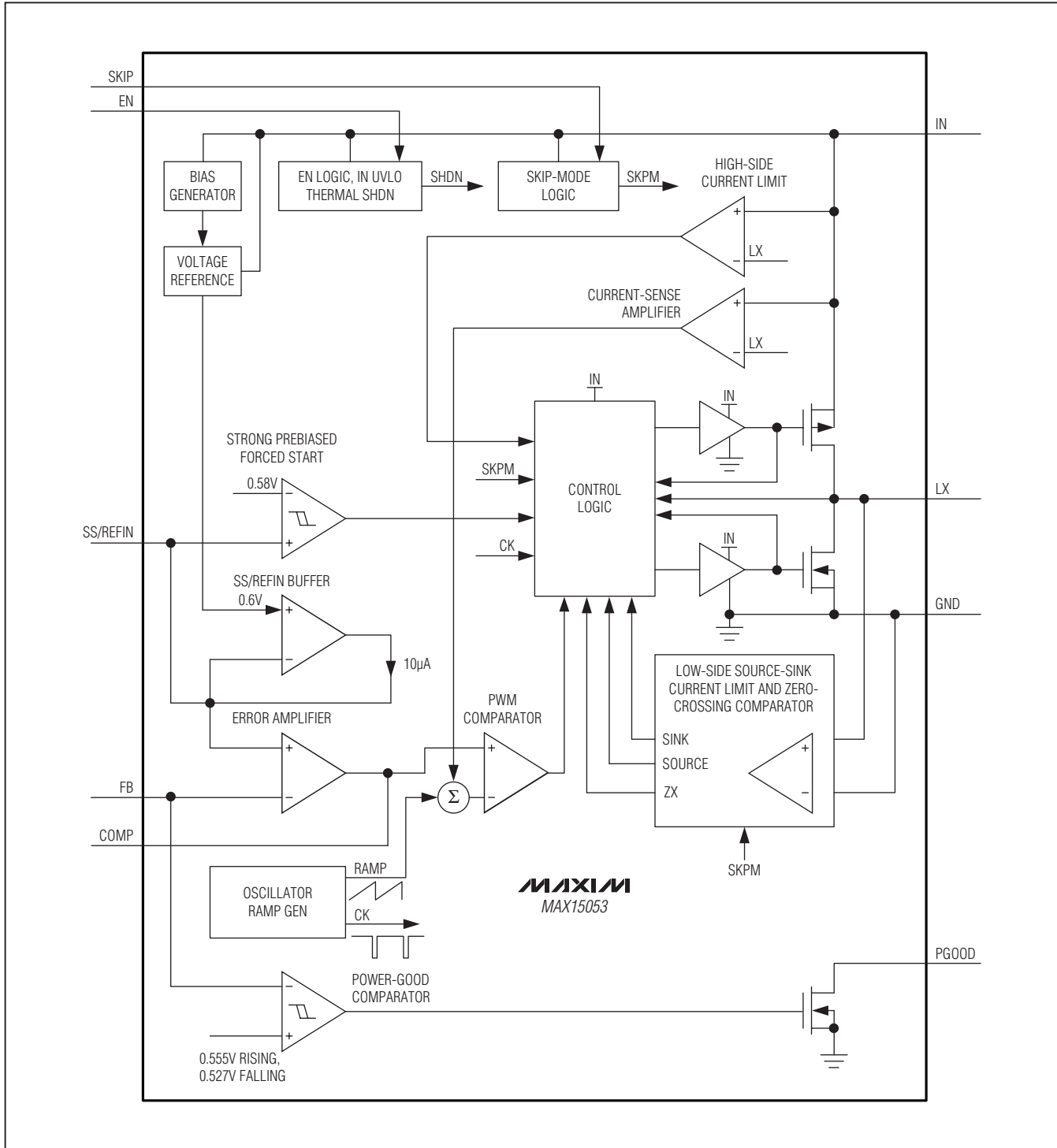
Block Diagram
