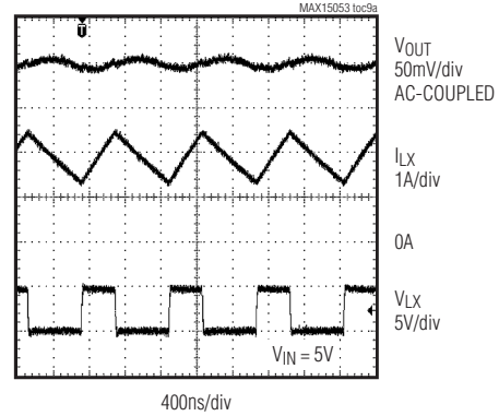
SWITCHING WAVEFORMS ( I_{OUT} = 2A )
