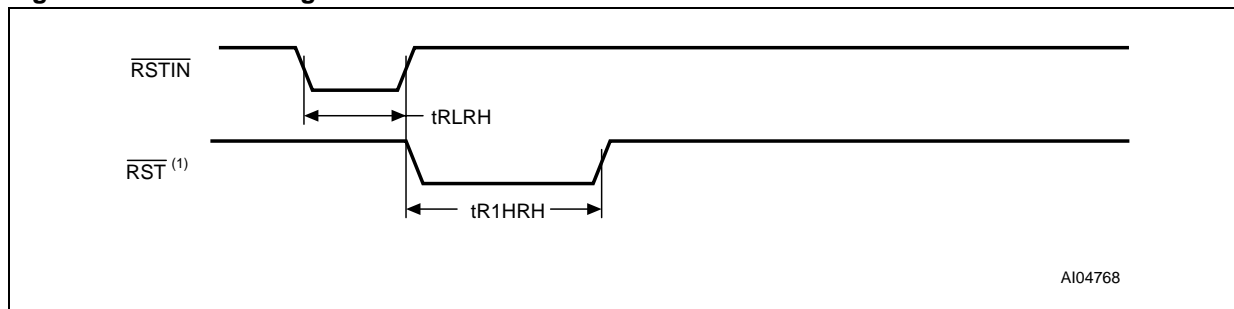
Figure 12. \overline{RSTIN} Timing Waveform
