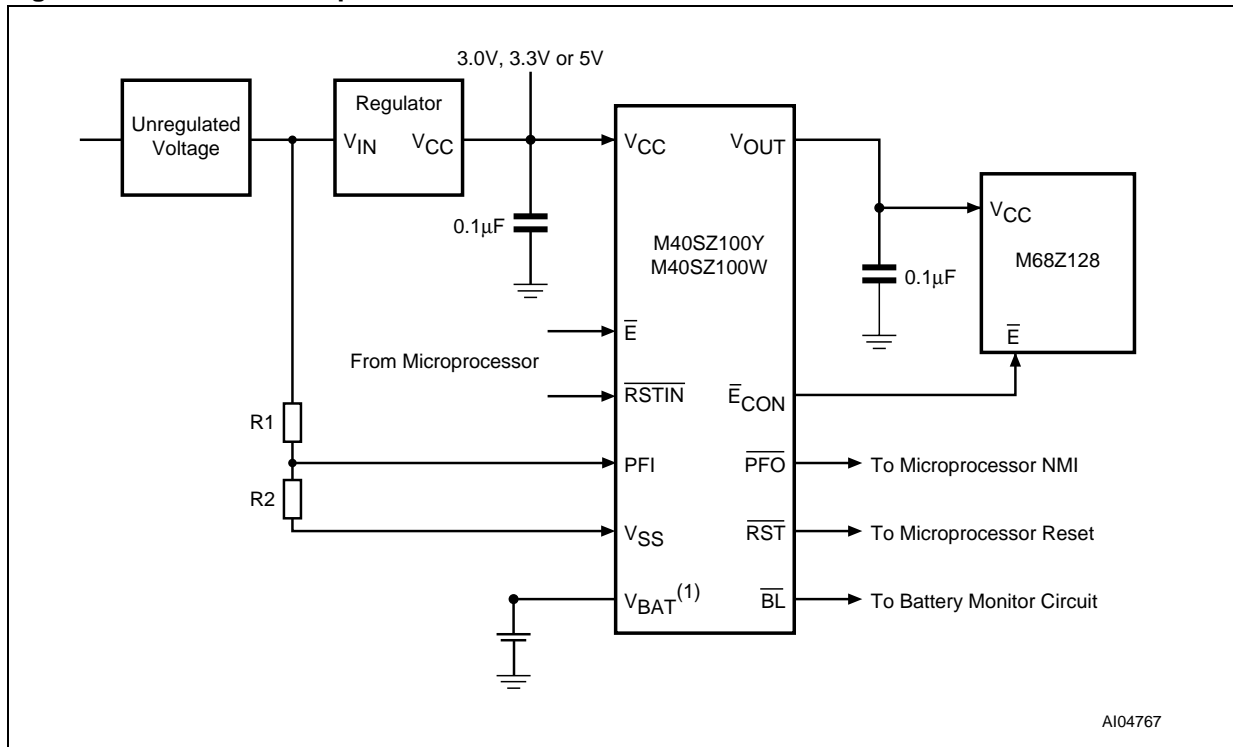
Figure 7. Hardware Hookup
