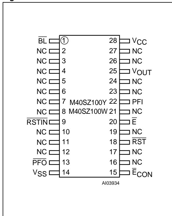
Figure 5. SOIC28 Connections
