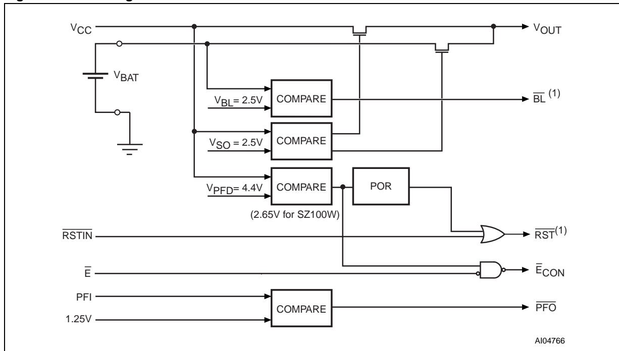
Figure 6. Block Diagram
