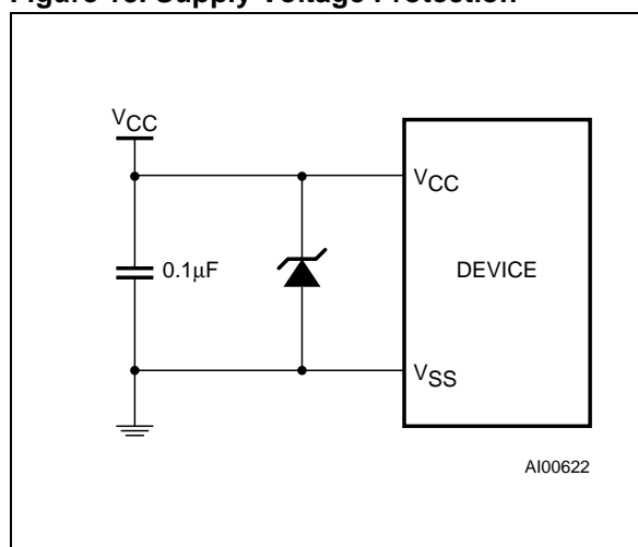
Figure 13. Supply Voltage Protection
