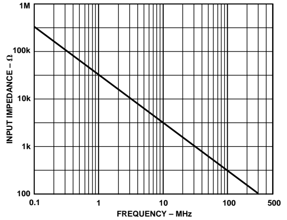
Figure 21. AD8115 Input Impedance vs. Frequency
