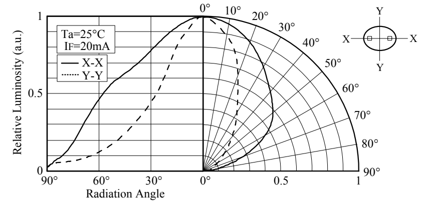
■ Directivity (NSPB346BS)
