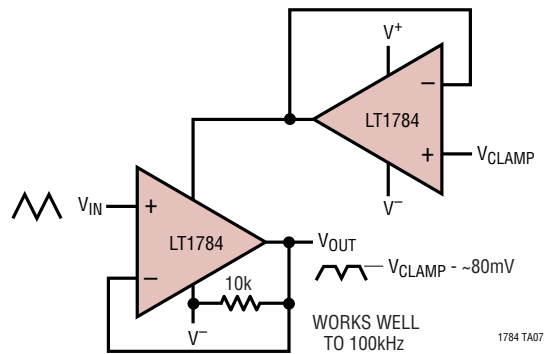
Adjustable Clamp
