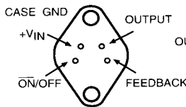
4-LEAD TO-3 (K)
