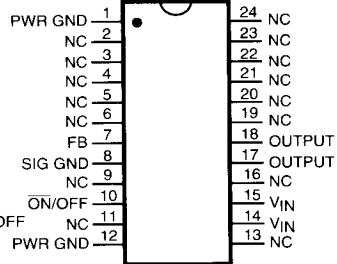
24-LEAD SOIC (WM)
