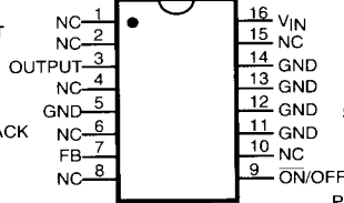
16-LEAD DIP (N)
