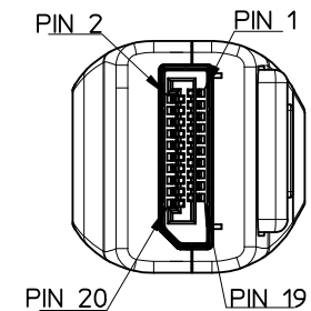
DETAIL PINOUT
