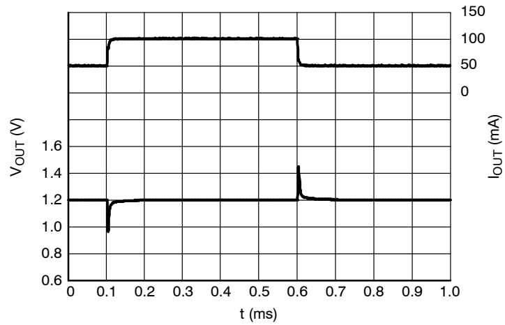
Figure 43. Load Transients, 1.2 V Version, I_{OUT} = 50 - 100 mA, t_R = t_F = 0.5 \mu\text{s} , V_{IN} = 2.2 V
