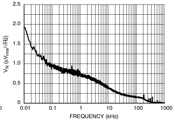
Figure 32. Output Voltage Noise, 2.5 V Version, V_{IN} = 3.5 V
