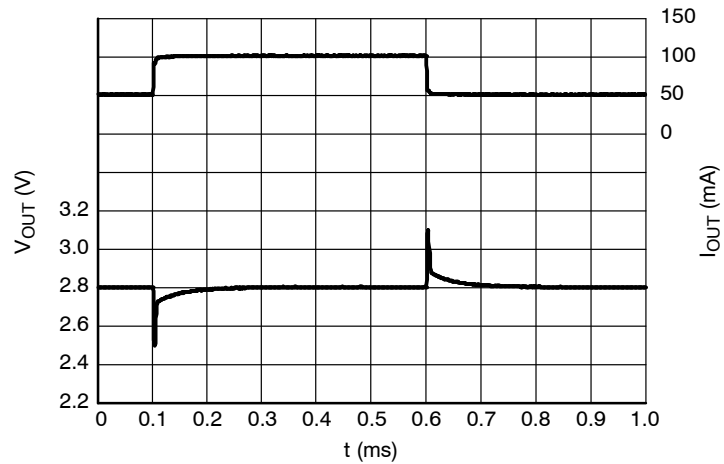
Figure 45. Load Transients, 2.8 V Version, I_{OUT} = 50 - 100 mA, t_R = t_F = 0.5 \mu\text{s} , V_{IN} = 3.8 V
