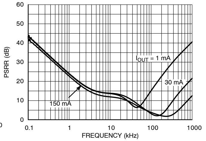
Figure 28. PSRR, 2.5 V Version, V_{IN} = 3.5 V
