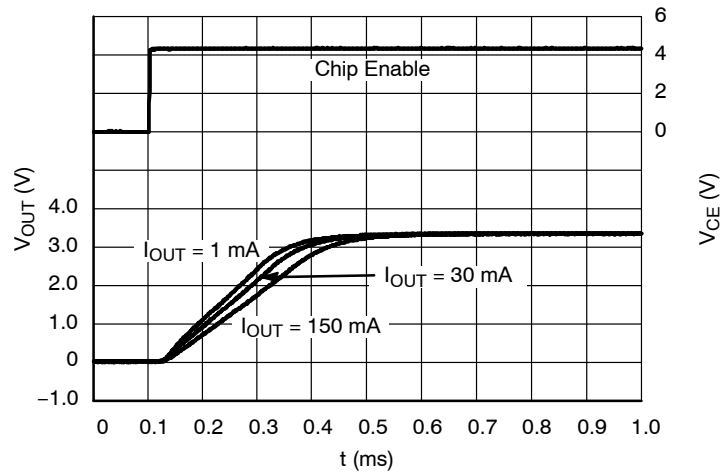
Figure 53. Start-up, NCP4682 3.3 V Version, V_{IN} = 4.3 V
