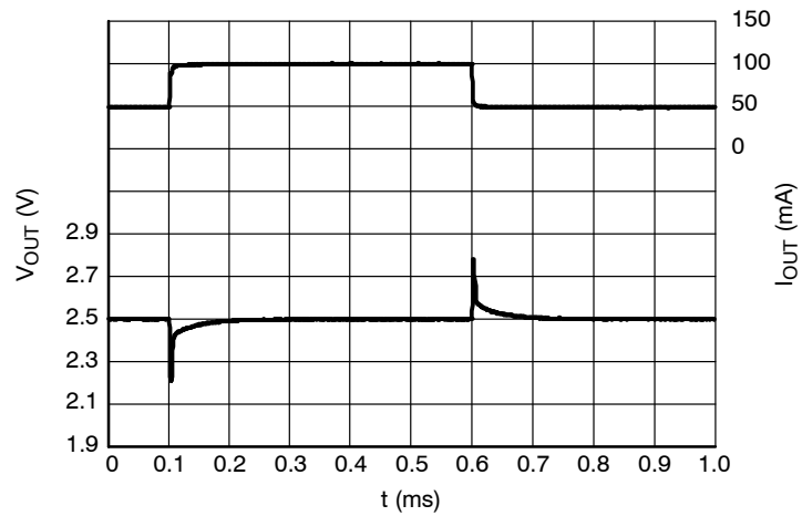
Figure 44. Load Transients, 2.5 V Version, I_{OUT} = 50 - 100 mA, t_R = t_F = 0.5 \mu\text{s} , V_{IN} = 3.5 V
