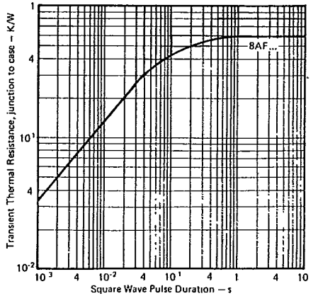
Fig. 18 — Maximum Transient Thermal Impedance, www.DataSheet4U.com Pulse Duration, 8AF Series
