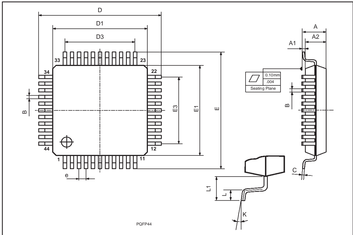
PQFP44 (10 x 10)
