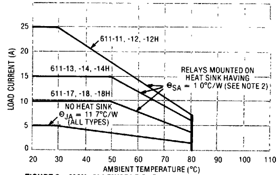
FIGURE 2 - MAX. ALLOWABLE CURRENT VS. AMBIENT TEMPERATURE
