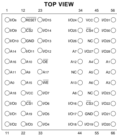
FIG. 1 PIN CONFIGURATION FOR WEDF1M32B-XHX5
