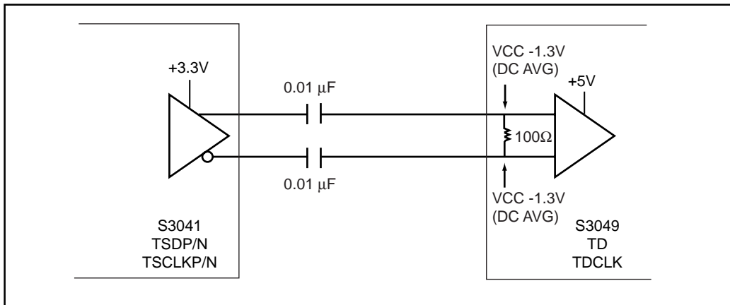
Figure 13. S3041 CML Output to +5V PECL Input AC Coupled Termination
