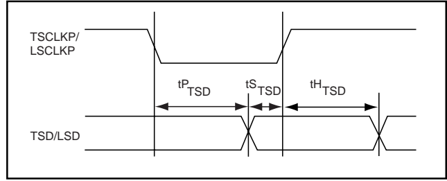
Figure 10. Output Timing
