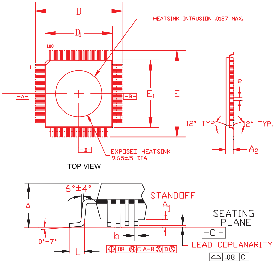
Figure 6. 100 TQFP/TEP Package
