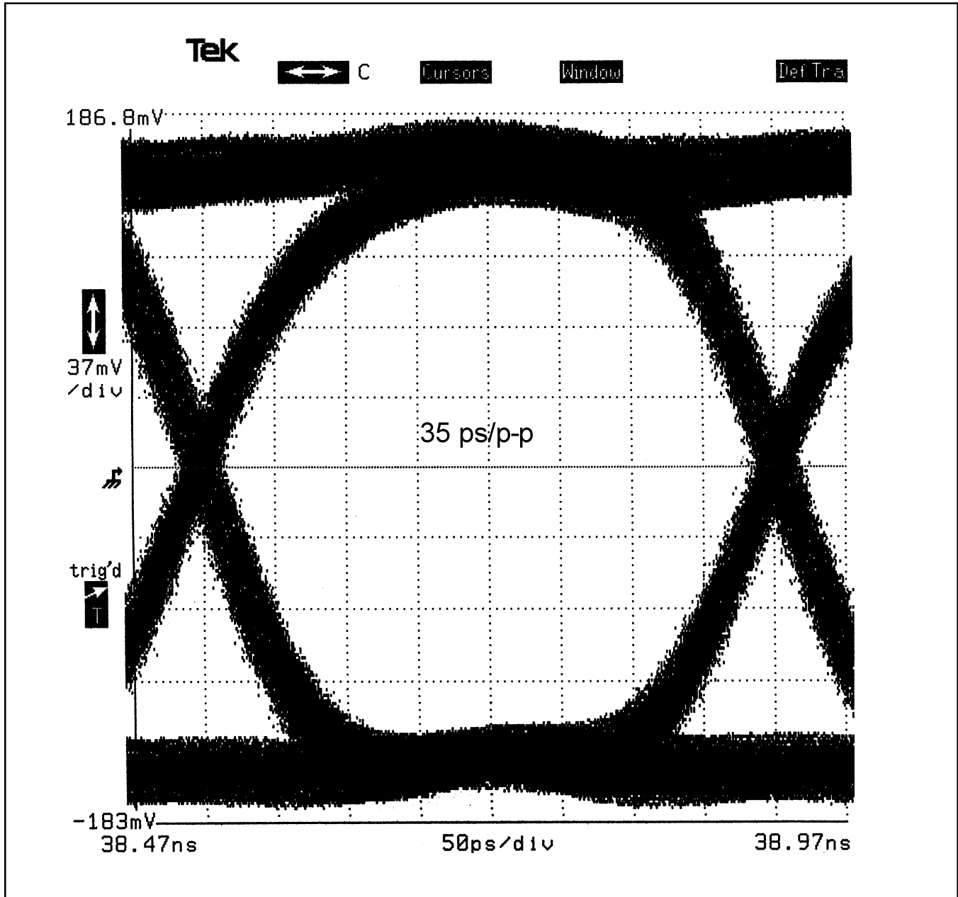
Figure 20. Typical Eye Opening for TSD
