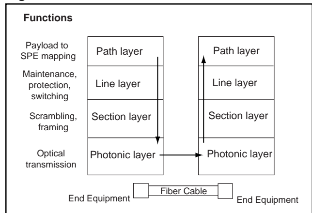
Figure 3. SONET Structure
