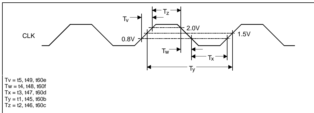
Figure 4. Clock Waveform
