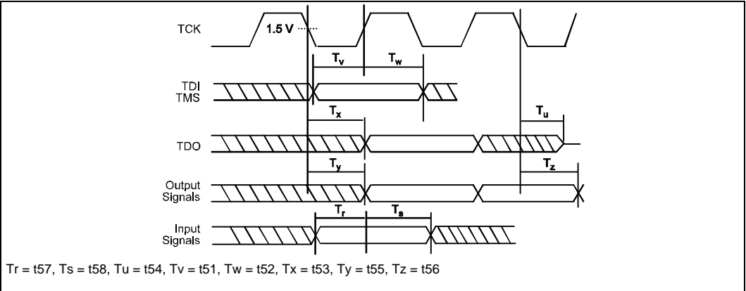
Figure 9. Test Timings
