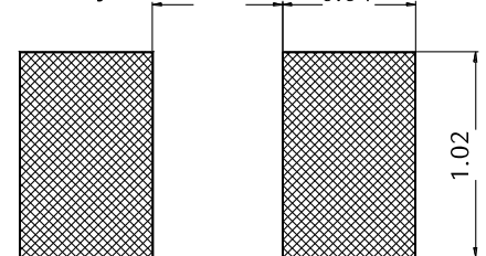
Pad layout
