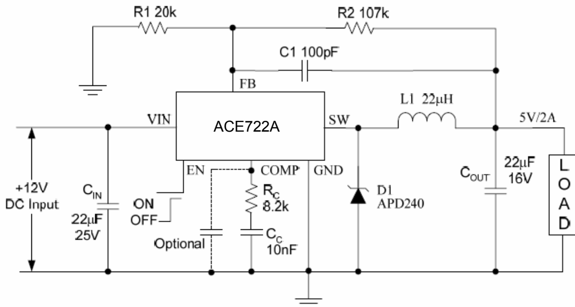
Figure 11. Typical Application 1 of ACE722A Applied with Ceramic Input and Output Capacitors
