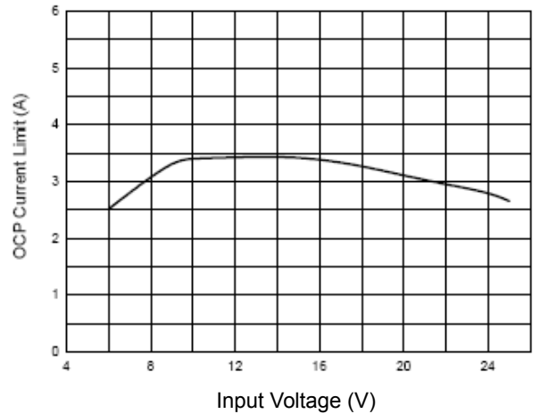
Figure 8. OCP Current Limit vs. Input Voltage
