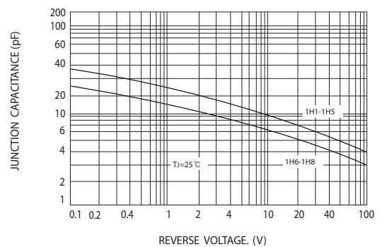
FIG.6-TYPICAL JUNCTION CAPACITANCE
